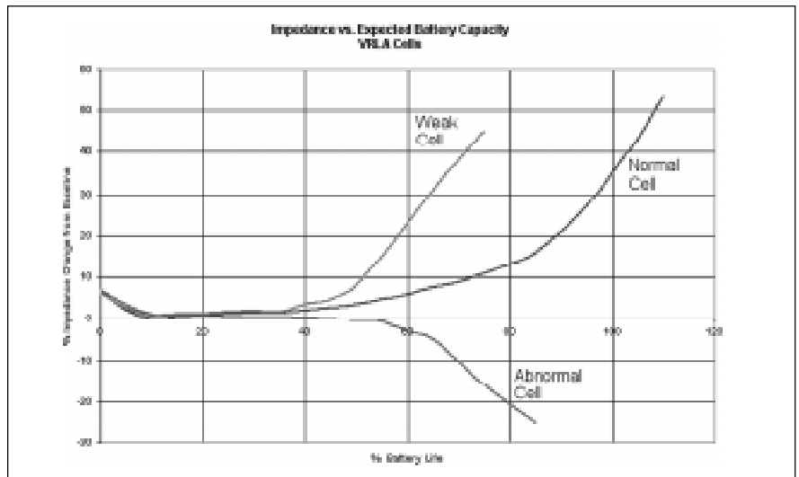
Figure 2. Impedance increases with battery age (and weakness).
