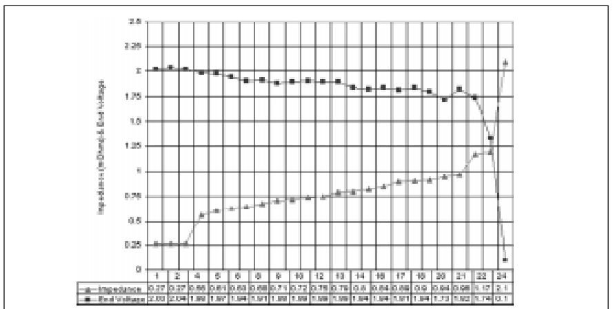
Figure 4. Ascending impedance compared to load test
