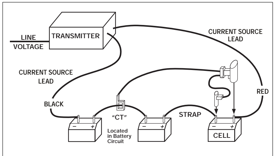
Figure 3. A typical test setup.
