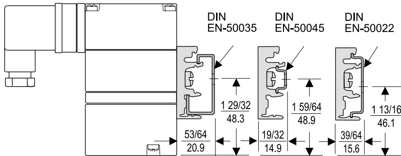
Figure 11. Din Rail Mounting Kit EA-16893-1. (Included with Unit)
