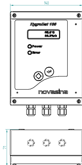
Version : "AL" Aluminium housing
