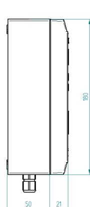
Version : "AL" Aluminium housing
