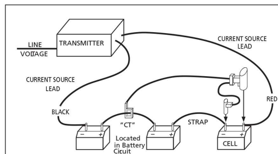
Figure 2. A typical test setup
