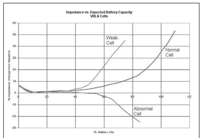
Figure 4. Impedance increases with battery age (and weakness)
